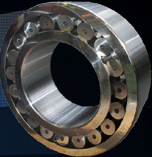
Large size spherical roller bearings with outside diameter up to 1600mm
