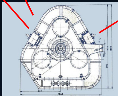
Planetary transmission of drive of belt
